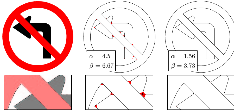
Fig. 3. Reconstructions before (red and black) and after (black only) thinning (note edges in lower left image). Connectivity errors can occur when \alpha is too big (center).
