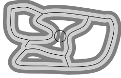
Fig. 1. The homotopy type of an r -stable plane partition does not change when dilated with a disc of radius of at most r (light gray), while dilations with bigger radius (dark gray) may connect different arcs as marked by the circle.
