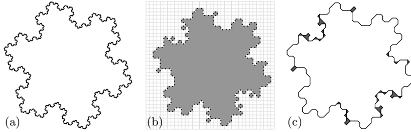
Fig. 7. (a) Koch Snowflake; (b) subset digitization (note the topology violations); (c) (\alpha, \beta) -boundary reconstruction from marked midcrack edgels. Areas where the edgels do not unambiguously determine the boundary shape pop out by remaining thick.
