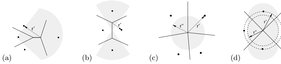
Fig. 6. Examples where the topology of the reconstruction by an r -grid (balls and lines) differs from the topology of the original set (gray area) because it is not r -regular.
