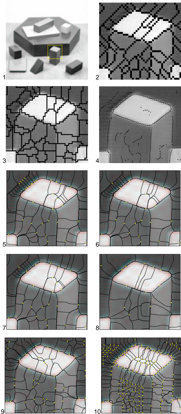
Figure 3. Evaluation of the exact watershed algorithm. 1) original image, ROI marked in yellow; 2) pixel-based watersheds of b_1 ( \sigma = 1.6 ); 3) inter-pixel (crack edge) watersheds of b_1 ; 4) Canny edgels from Gaussian gradient with \sigma = 1.6 ; 5 to 9) exact watersheds: 5) order 2 interpolation of b_1 ; 6) order 3 interpolation of b_1 ; 7) order 5 interpolation of b_1 ; 8) dto. for b_3 ( \sigma = 1.1 , \sigma' = 2.2 ); 9) dto. for b_4 ( \sigma = 1.1 ); 10) dto. for b_5 (window radius = 3.4, \gamma = \|\mathcal{W}\| , \delta = 15 ). Maxima of the boundary indicators are marked in yellow.
