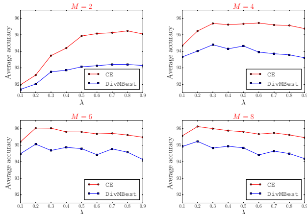
Figure 4: Pixelwise accuracy comparison for interactive segmentation for different values of \lambda and M .
