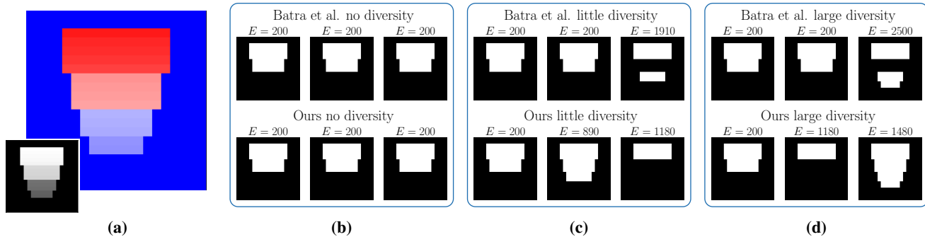
Figure 1: Comparing our approach to Batra et al. [4] for a toy image. (a) the unary terms of the energy (red/blue means more likely fore-/background). The Inlet shows the original image. (b-d) Results for three different levels of diversity. For each diversity level we ask for three output images, where E is the associated energy. (b) Both methods produce three times the same MAP solution. (c) When forcing diversity both methods give different results. Note that the sum of the pairwise Hamming distances between the results is the same for both methods. However, our result is visually better, since it contains solutions that are more coherent. This is also reflected in the energy. The sum of the energy of the three solutions is lower with our method (2270 compared to 2310). Our method directly optimizes for this energy. (d) When forcing strong diversity, the set of solutions becomes more diverse for both methods. Again, our result is superior, visually and in terms of total energy, while both results have the same overall Hamming distance.
