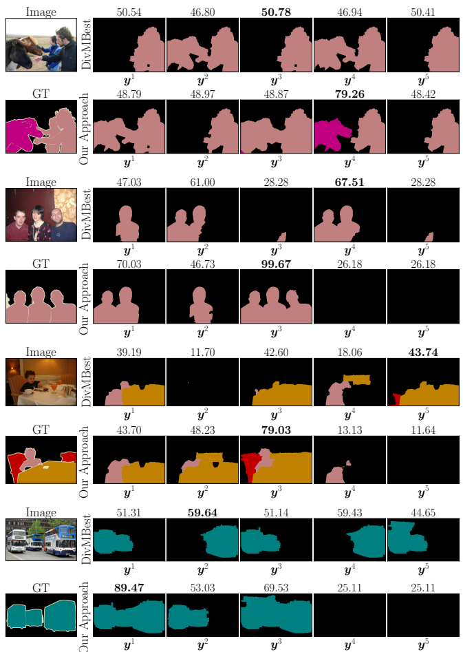
Figure 6: Comparison for samples from Pascal VOC 2012 dataset. Number above each solution is a corresponding intersection over union quality measure.
