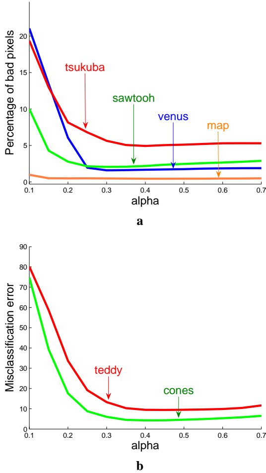
Fig. 21. Sensitivity to parameters. (a) Sensitivity of the “percentage of bad pixels” error metric with respect to \alpha . Note the flat behaviour for \alpha > 0.35 . (b) Sensitivity of occlusion misclassification rate with respect to \alpha . In all cases errors are measured on standard Middlebury stereo pairs. Occlusion errors are measured on the two stereo pairs with the largest occlusions. 4-state DP is not particularly sensitive to values of \alpha varying within a reasonable range.
