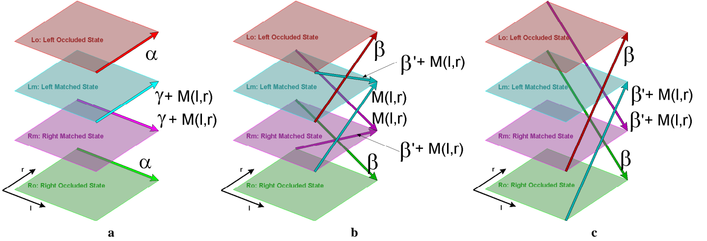
Fig. 10. The proposed four-state model for DP. The graph associated with our new DP algorithm occupies four planes, with 14 allowed state transitions: (a) state-preserving transitions and (b,c) between-state transitions. Each permitted state transition (shown by arrows) has been labelled with the associated cost — see text.
