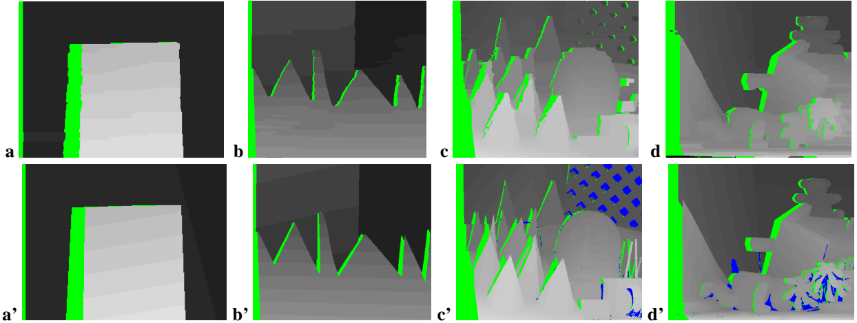
Fig. 18. Accuracy of occlusion estimation on Middlebury stereo pairs. (a-d) Estimated occlusions and disparities for the left view of Map, Sawtooth, Cones and Teddy pairs, respectively. (a'-d') Corresponding ground-truth occlusions and disparities (blue denotes unlabelled pixels). Good correspondence between the ground-truth occlusions and those estimated by 4-state DP is evident. Measured occlusion detection accuracy \left( \frac{n. \text{ correctly detected occlusions}}{n. \text{ all detected occlusions}} \right) for the four cases is: (a) 93%, (b) 90%, (c) 79%, (d) 85%. The maximum occlusion gap of 55 pixels (12% of image width) occurs at the edge of the Cones image. The maximum occlusion for Map is about 9% of the image width.
