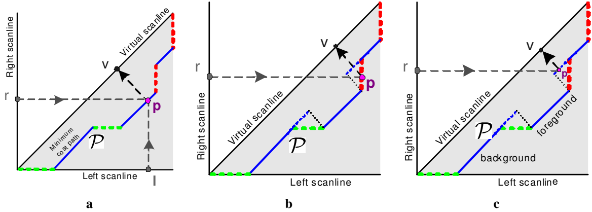
Fig. 7. Generating the cyclopean view. (a) A matched point p \in \mathcal{P} is projected orthogonally onto its corresponding point v on the virtual scanline. The luminance value of the virtual pixel v is the average of the corresponding pixels l and r on left and right images, respectively. (b) Halo : treating the occluded segments (dotted lines) in \mathcal{P} in the same way as the matched segments produces a lens-like effect that we call the “halo” artefact (fig. 8). (c) Fronto-parallel occlusion synthesis : the halo effect is largely removed if a fronto-parallel background assumption is made: an occluded point p on the continuation of the background is projected orthogonally onto its corresponding point v on the virtual scanline.
